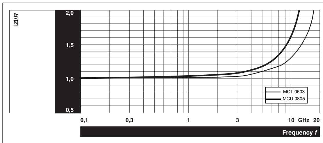
Fig.9 |Z|/R for 49,9 Ω chip resistor.
